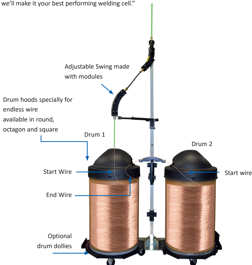
Single torch unit (with round drums)
